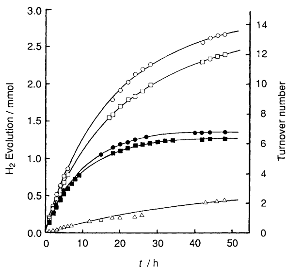
Figure 1. Time-course plots of \text{H}_2 evolution from the cyclo-octane solution (0.2 mmol metal/100 ml) of \text{RhCl}[\text{P}(p\text{-tolyl})_3]_3 (○), \text{RhCl}(\text{PPh}_3)_3 (□), [\text{RhCl}\{\text{P}(p\text{-tolyl})_3\}_2]_2 (●), [\text{RhCl}(\text{PPh}_3)_2] (■), and \text{RhCl}(\text{PMePh}_2)_3 (△) under boiling and refluxing conditions (151 °C).
